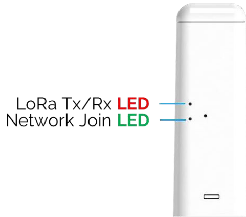
Figure 2-7: FINCH LEDs
