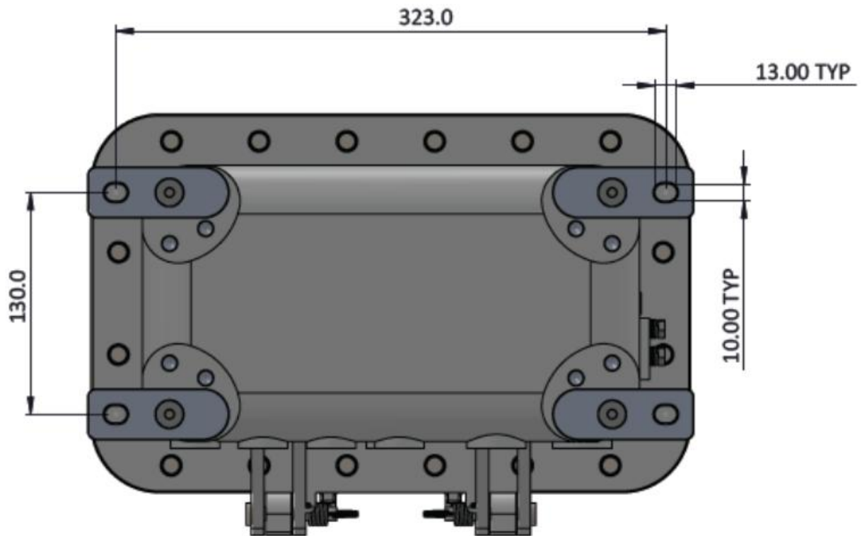
Figure 4: Kona Macro Ex Mounting Hardware Location, 0° Tab Orientation
