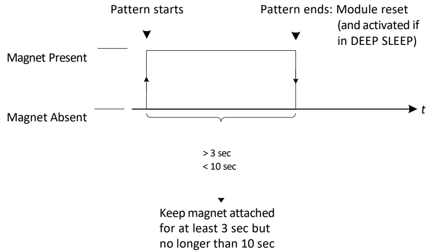
Figure 2-1: The C-Cell Tracker Variant Magnetic Activation Pattern
