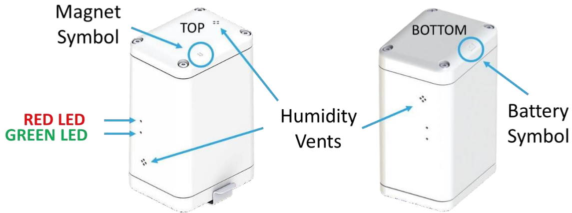
Figure 1-1: PELICAN Enclosures and External Interfacing
