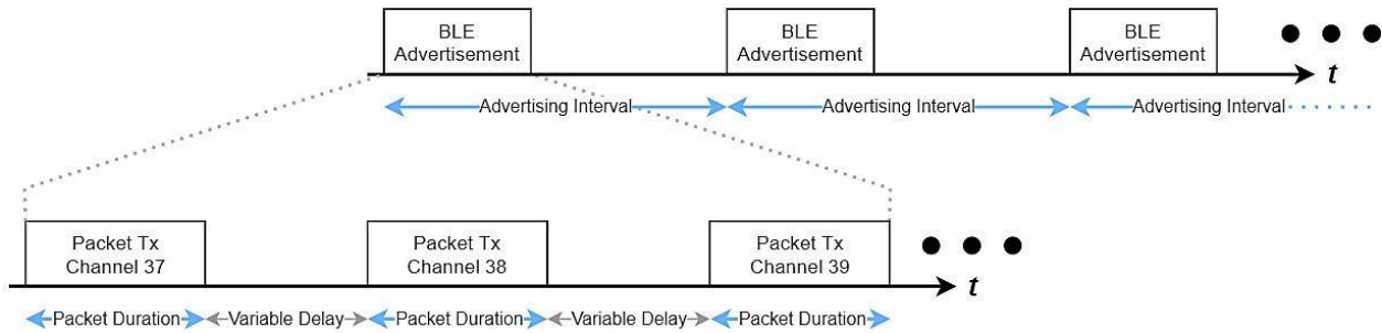
Figure 3-3: The BLE Advertising Scheme
